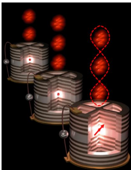
Artist's view of three single-photon sources showing the presence of a semiconductor quantum dot inside an optical microcavity, and emitting a series of single photons. When the quantum dot contains a single spin (in the foreground), entangled photons can be emitted. © Niccolo Somaschi, 2016.
