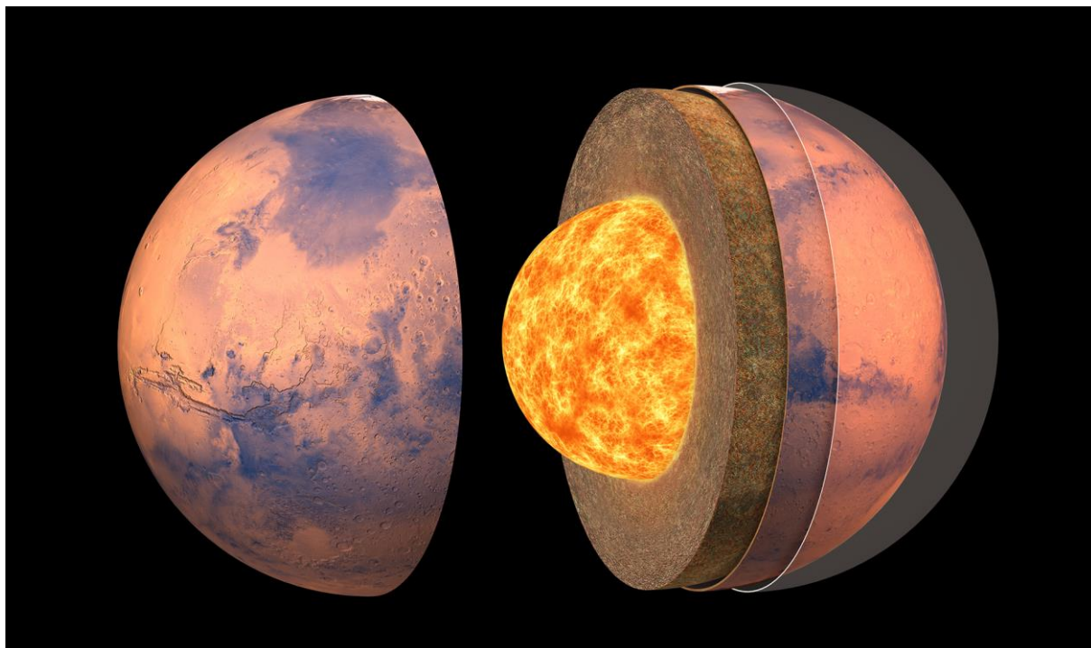
Artist's impression of the internal structure of Mars (© IPGP / David Ducros)
